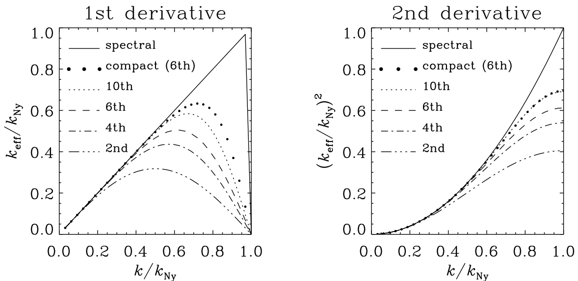
Figure 30: Effective wave numbers for first and second derivatives using different schemes. Note that for the second derivatives the sixth order compact scheme is almost equivalent to the tenth order explicit scheme. For the first derivative the sixth order compact scheme is still superior to the tenth order explicit scheme.
