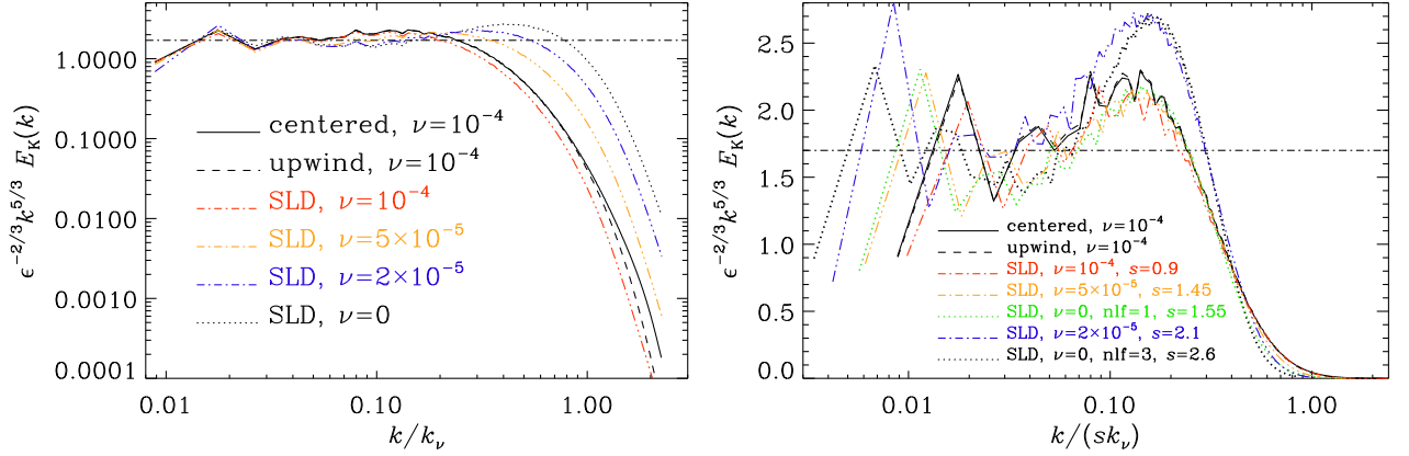
Figure 32: Comparison of centered (solid lines) and upwinding (dashed lines) advection in a 512^3 isothermal turbulence simulation forced with f_0 = 0.02 . The computational domain is L^3 with L = 2\pi and the forcing wavenumber is k_f = 1.5 . The viscosity is \nu = 10^{-4} . The dotted line gives a run without regular diffusion, but with slope-limited diffusion (SLD) instead. In the right panel, the curves are plotted versus k/(sk_\nu) , where k_\nu = (\epsilon_K/\nu^3)^{1/2} is the nominal viscous cutoff wavenumber, and s is an empirical gain factor that has been introduced to collapse the spectra in the inertial range. The maximum gain factor is 2.6, but at the price of increasing the bottleneck.
